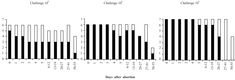
Figure 5. Assessment by PCR of the shedding of C. burnetii in milk the day of abortion and the following days. ■ positive PCR, □ negative PCR.
