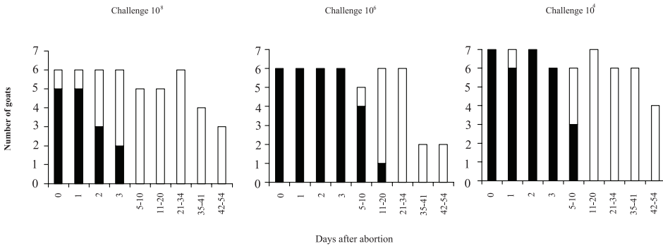
Figure 4. Assessment by PCR of the shedding of C. burnetii in vaginal swabs the day of abortion and the following days. ■ positive PCR, □ negative PCR.
