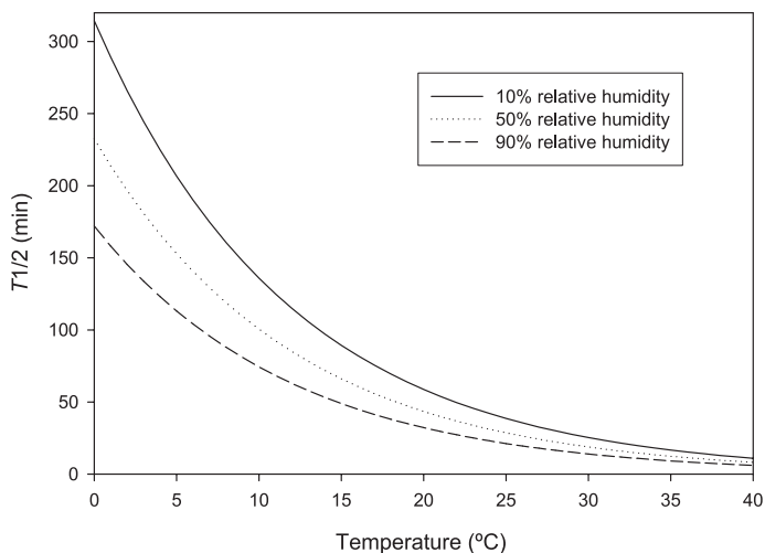
Figure 2. Predicted effect of temperature on half-life of aerosolized infectious PRRSV at 10%, 50%, and 90% relative humidity.
