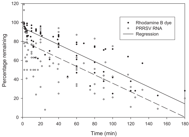
Figure 4. Percentage of Rhodamine B dye and PRRSV RNA remaining out of total aerosolized over time.
